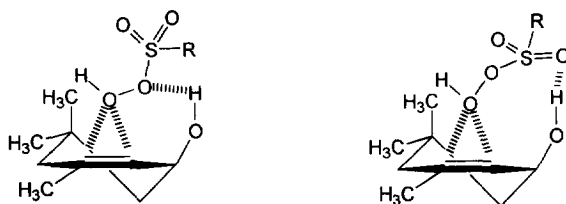
Possible transition states for the syn selective epoxidation by the sulfonic peracid 2
